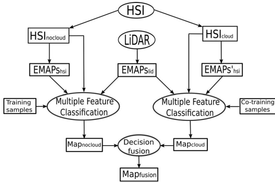
Fig. 3. Flowchart of the proposed framework, here HSI nocloud and HSI cloud denote the shadow-free and cloud-shadow regions of HS image, EMAP HSi and EMAP HSi mean MPs extracted from hyperspectral and LiDAR data. “Cotraining samples” are generated training samples by our methods for cloud-shadow regions.
