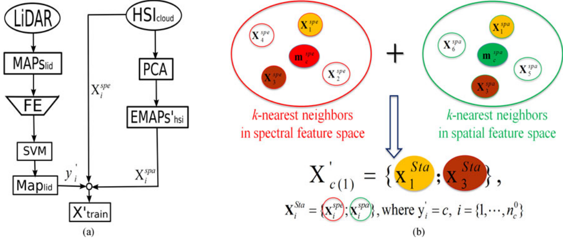
Fig. 8. (a) Cotraining samples selection; x_i^{spe} and x_i^{spa} represent spectral radiance and EMAPs hsi of the i th pixel; (b) x_i^{Sta} = \{x_i^{spe}; x_i^{spa}\} ; the pixel is labeled c in Map lid ( y'_i = c ); m_c^{spe} and m_c^{spa} are the centers of class c in spectral and spatial feature space, here x_1^{Sta} and x_3^{Sta} are the nearest neighbors of the center of class c , both in spectral and spatial feature space, and selected as candidate cotraining samples.
